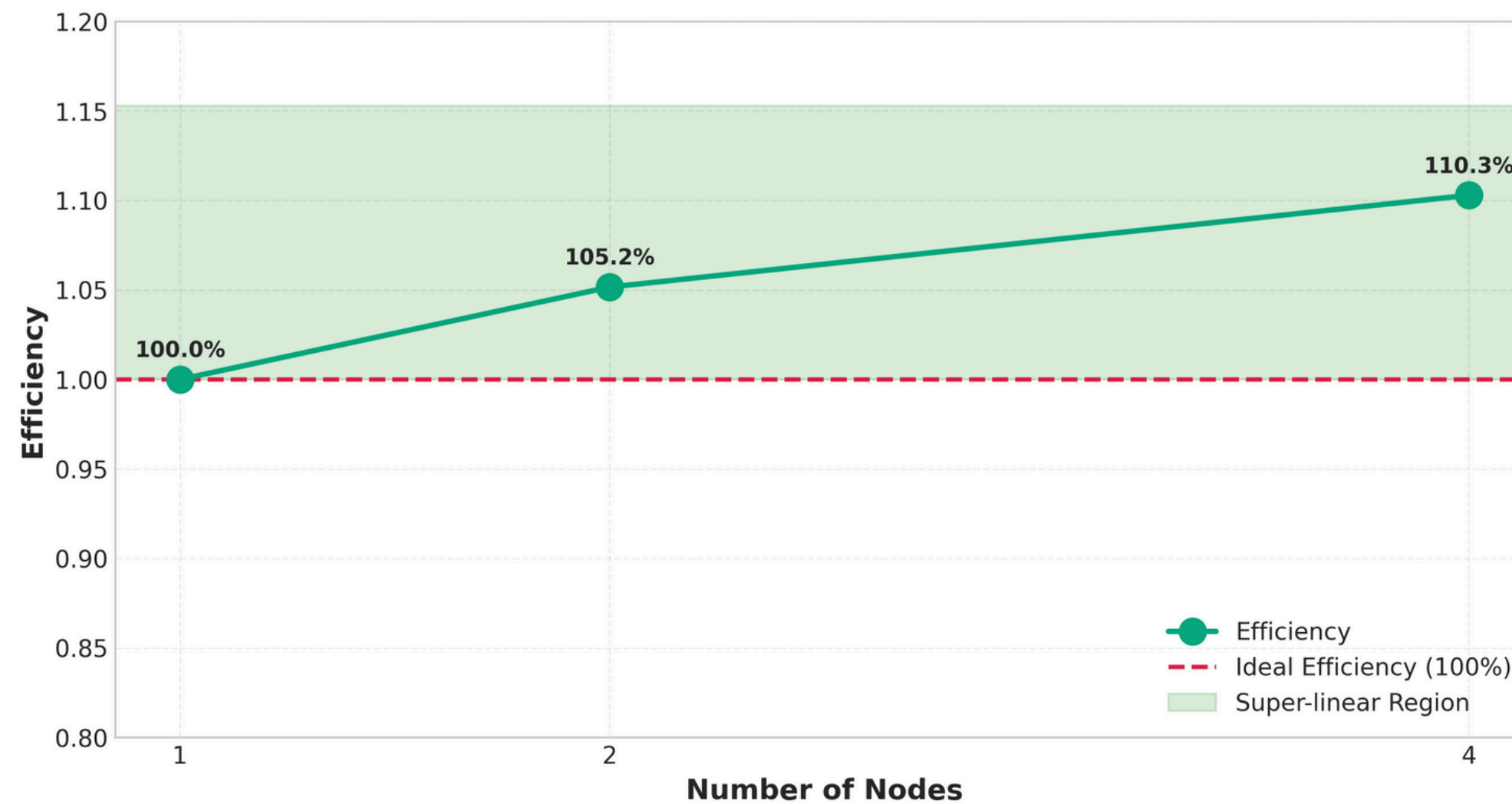
MPI Weak Scaling: Efficiency vs Nodes ~2000×2000 per Node, 128 Threads/Node
